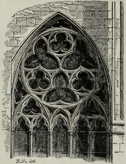
122. Passage to the Chapter-house, York, c. 1260—1280. Shewing geometrical tracery.
